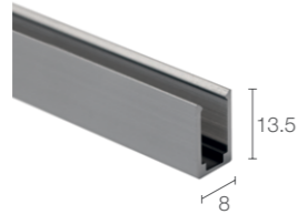
WDA14 - 1000 mm Profilo in alluminio Profile in aluminium
