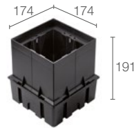
WCA15 Outer casing (Quilatero 3)
