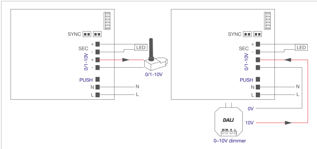
0/1-10V control
