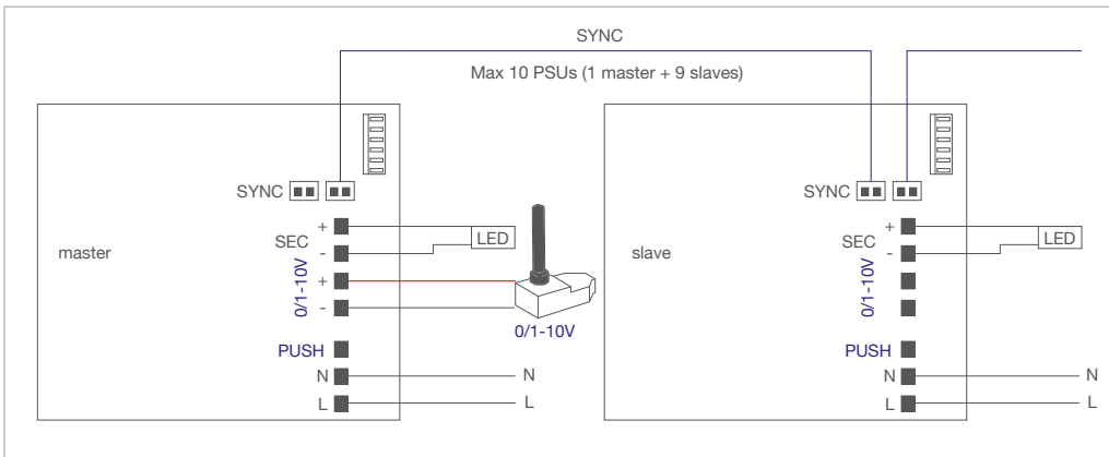
0/1-10V control with synchronization with ADUNITC
