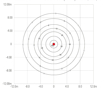
RR - Radiale 360° / Radial 360° (H 3m) Isolux (3000K)
