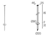
WP1007E Spike for in-ground installation - h 800 mm - white
