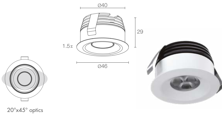
20°x45° optics
